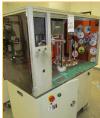
PHONEBIRD #ID-1500 DISC ID CHECKER
